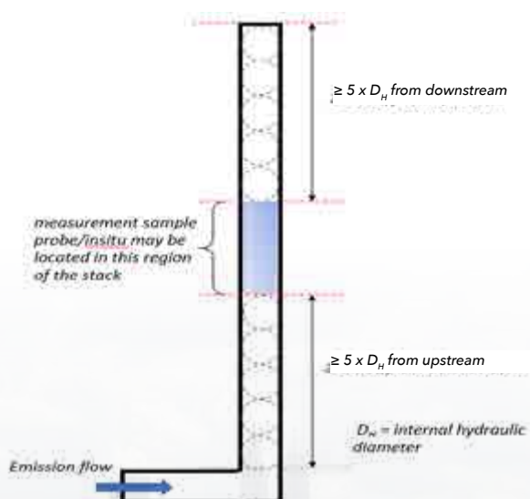
Figure 4.1 - Sampling probe location
